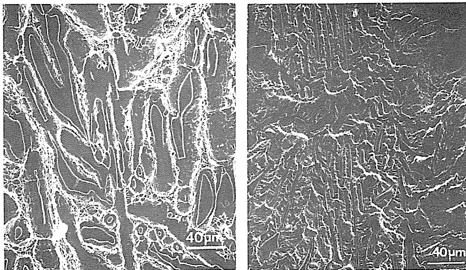
FIG. 7 -- Scanning electron microscope fractographs exhibiting MnS inclusion clusters on SL oriented CVN specimen (left) and SL oriented FCP sample (right).
