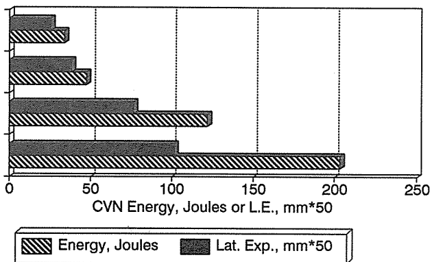
FIG. 10 -- Improvements made to A553 steel and enhancements to CVN properties.
